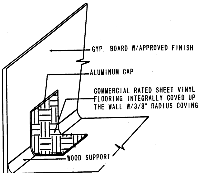
TYP. COMM. SHEET VINYL DETAIL
