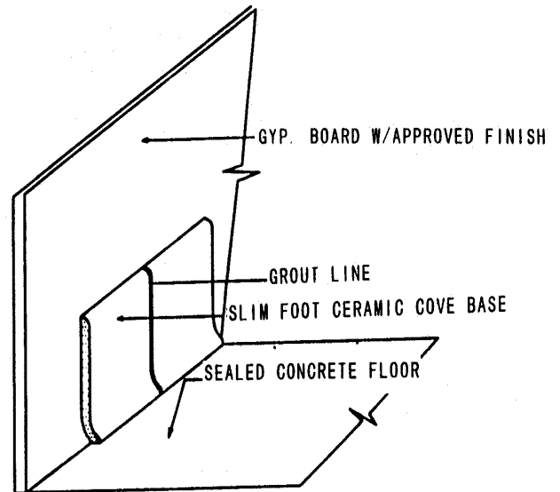
TYP. CERAMIC 'SLIM-FOOT' ON CONCRETE
