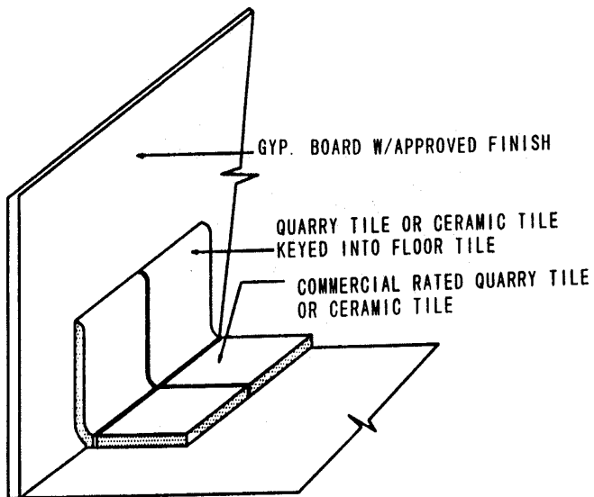
TYP. CERAMIC OR QUARRY TILE DETAIL
